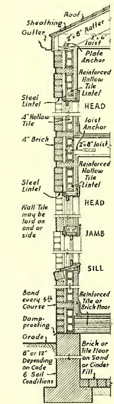
Wall Section
